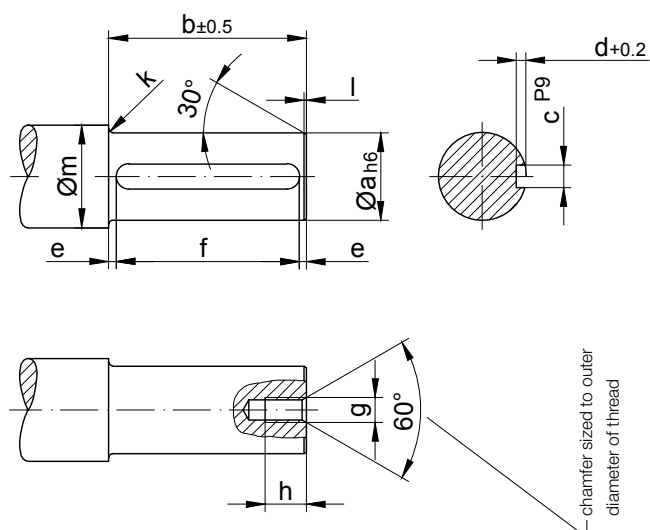
Position 1 Shaft
