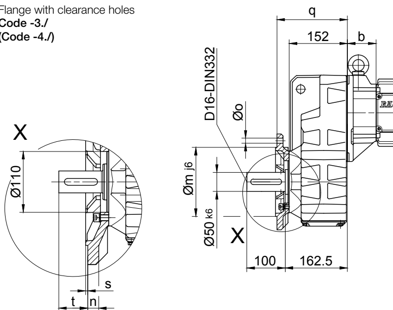
Flange Dimensions
