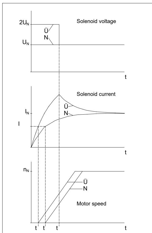
Figure 3: Idealised curves of coil voltage, coil current and motor speed with normal excitation (N) and overexcitation ( \ddot{U} ).
