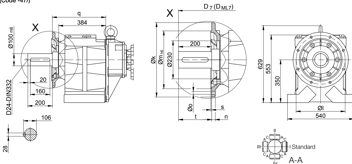
Flange Dimensions
