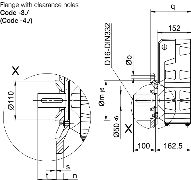
Flange Dimensions
