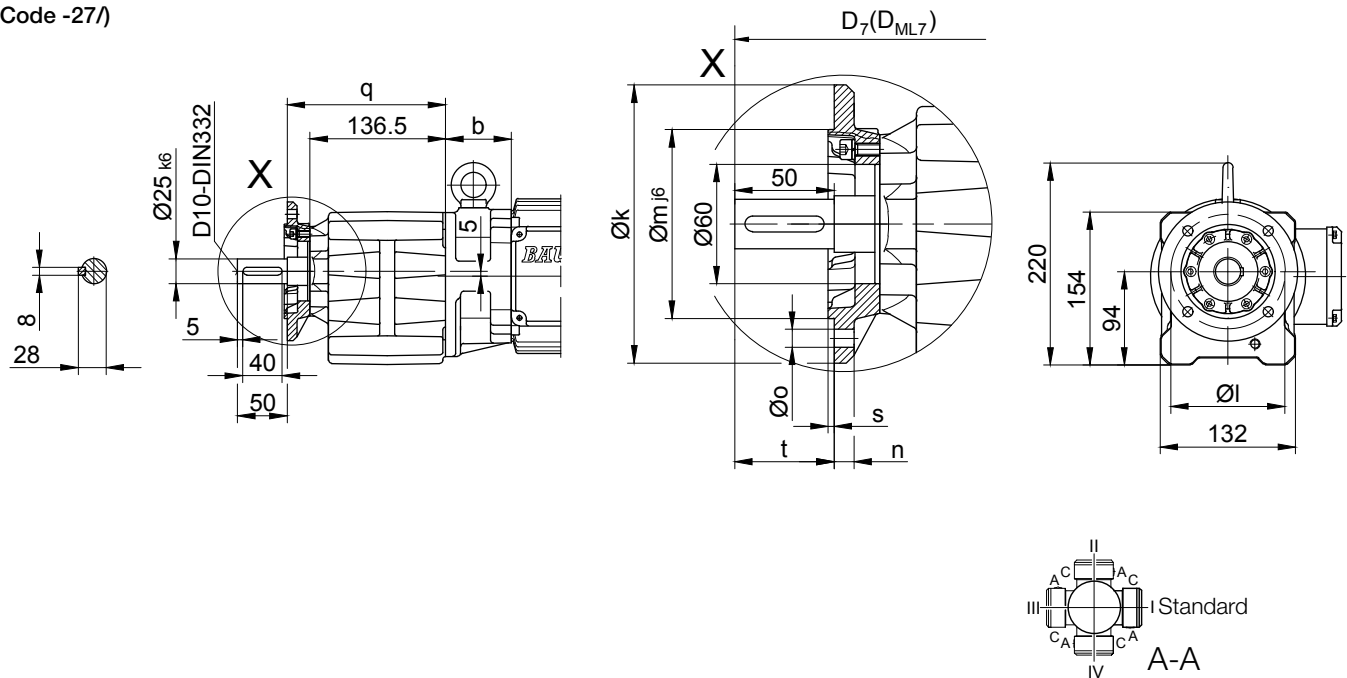
Flange Dimensions
