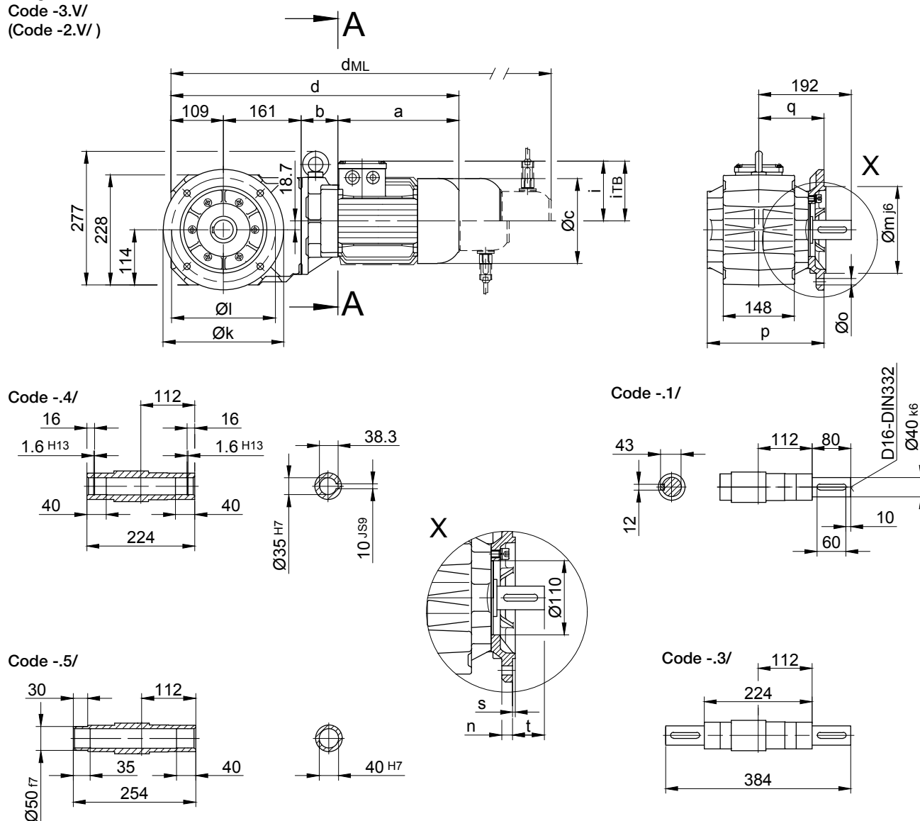
Flange Dimensions
