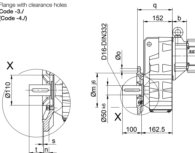
Flange Dimensions
