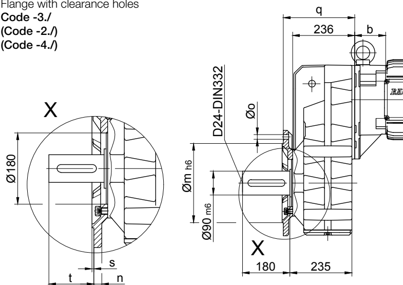
Flange Dimensions
