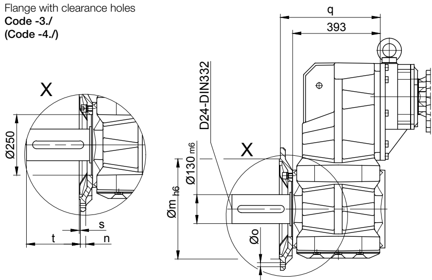
Flange Dimensions
