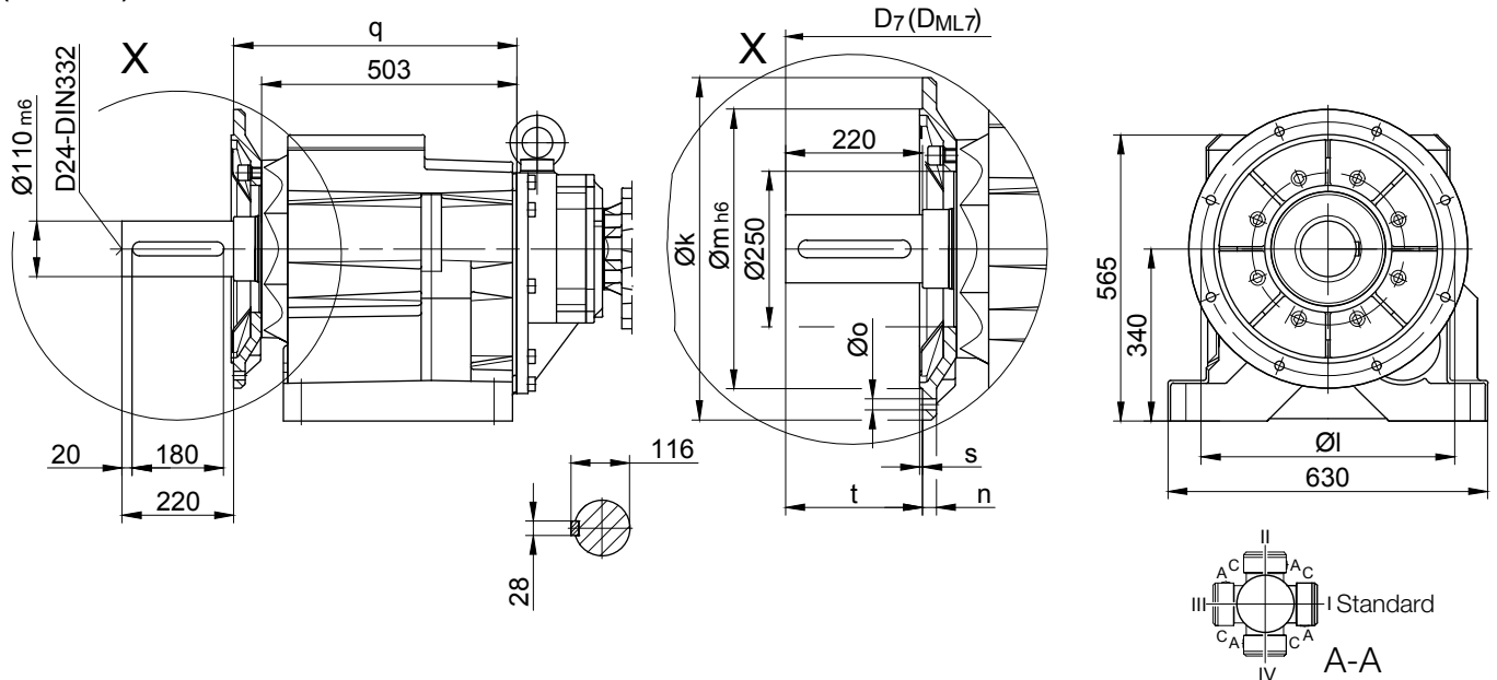
Flange Dimensions
