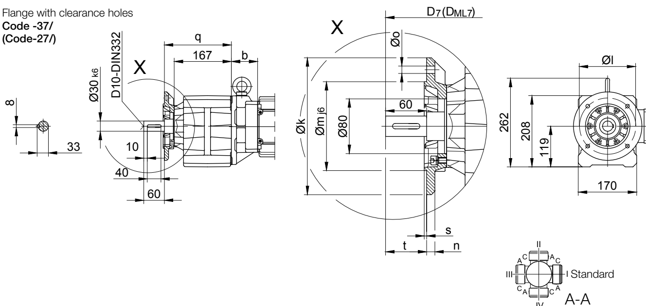
Flange Dimensions
